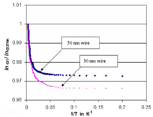
FIG. 3. Normalized temperature dependence of the conductivity of a single Bi nanowire with widths of 50 and 30 nm.
