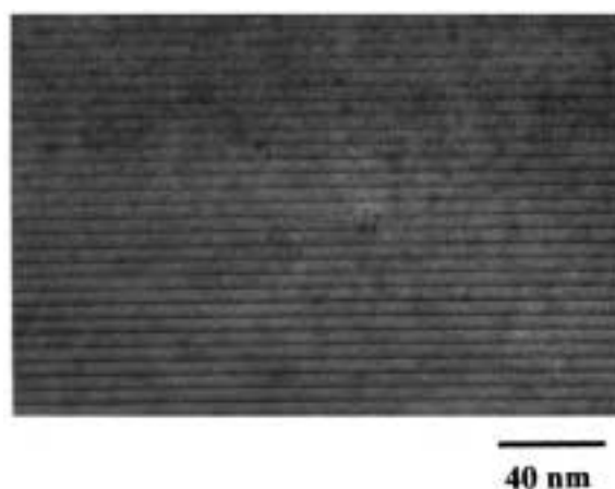
FIG. 1. Cross-sectional TEM image of the sample. The quantum dots can be seen as dark features distributed in the Ge wetting layer dark stripes.
